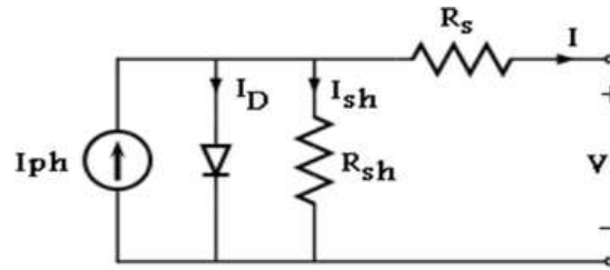
Figure 1. PV cell equivalent circuit
